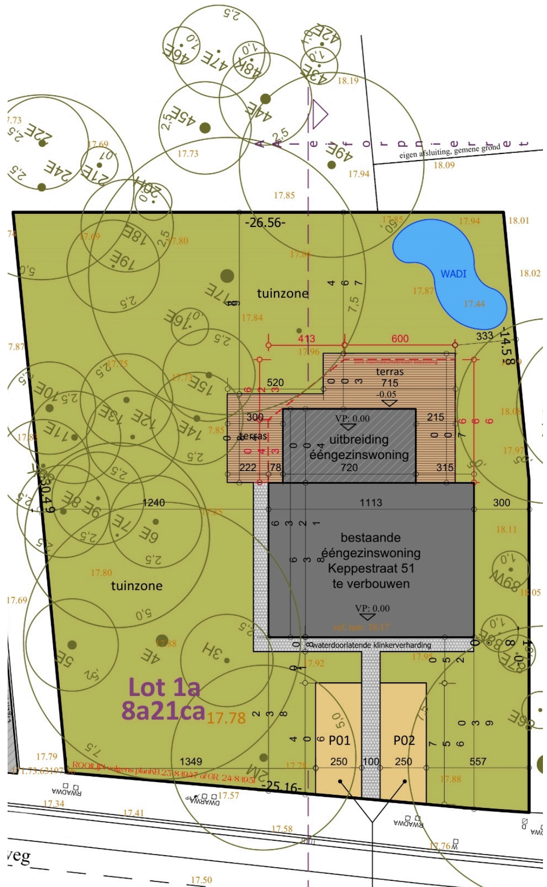
INPLANTINGSPLAN
